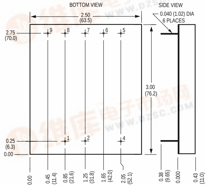
PIN CONNECTIONS
