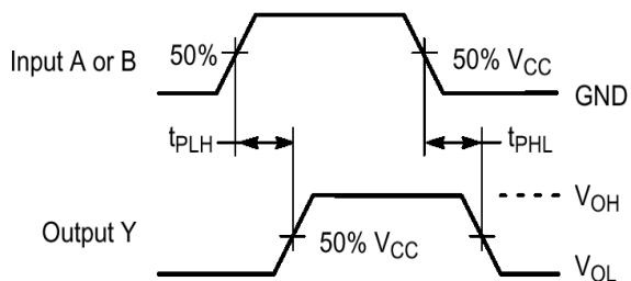
Figure 4. Switching Waveforms
