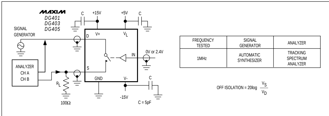
Figure 5. Off Isolation
