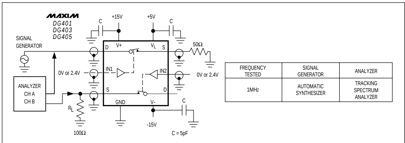
Figure 6. Crosstalk
