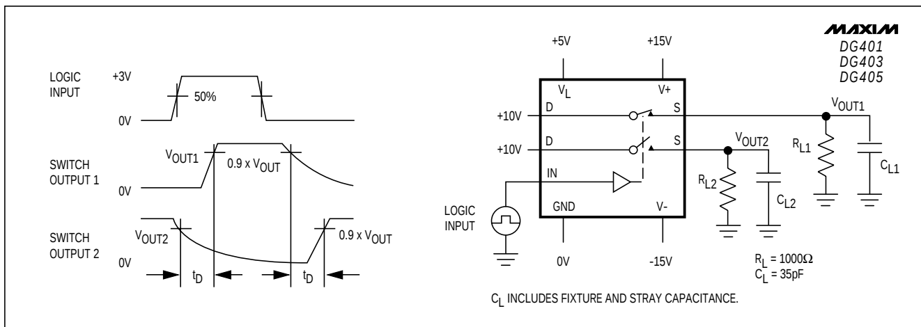
Figure 3. Break-Before-Make Interval
