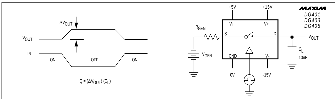
Figure 4. Charge Injection
