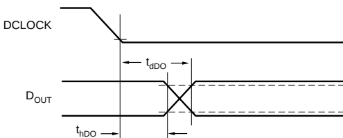
Voltage Waveforms for DOUT Delay Times, t_{dO}
