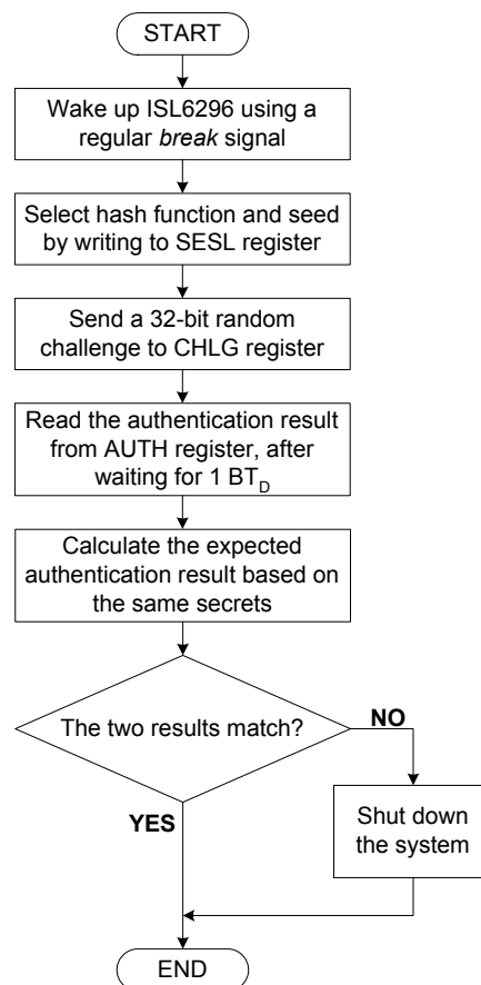
FIGURE 6. FLOW CHART FOR AUTHENTICATION PROCESS
