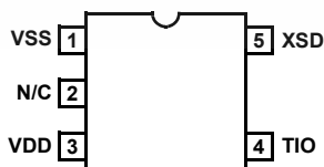
ISL6296 (SOT23-5) TOP VIEW
