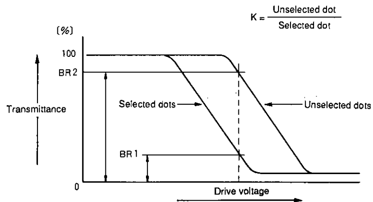
Figure 3 Contrast Definition
