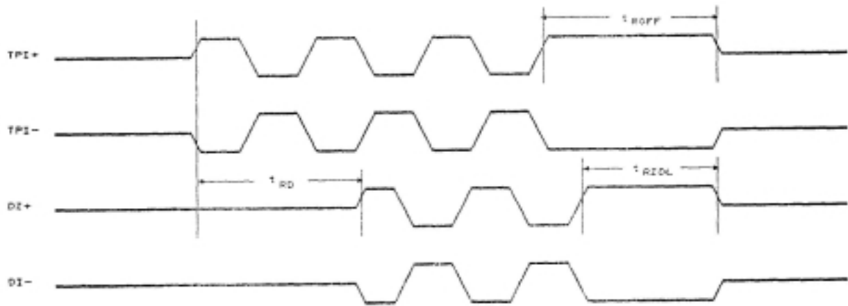
Figure 7. Receive timing
