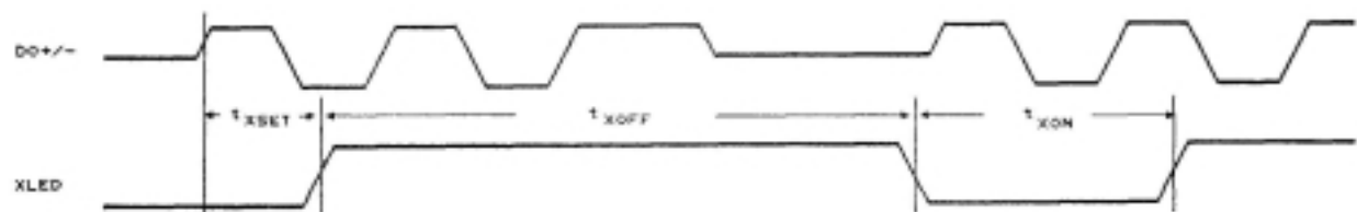
Figure 12. XLED timing
