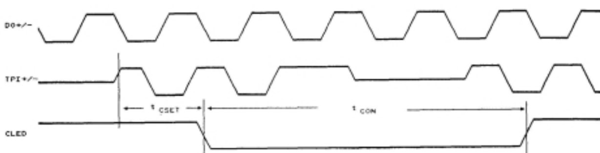
Figure 15. CLED timing
