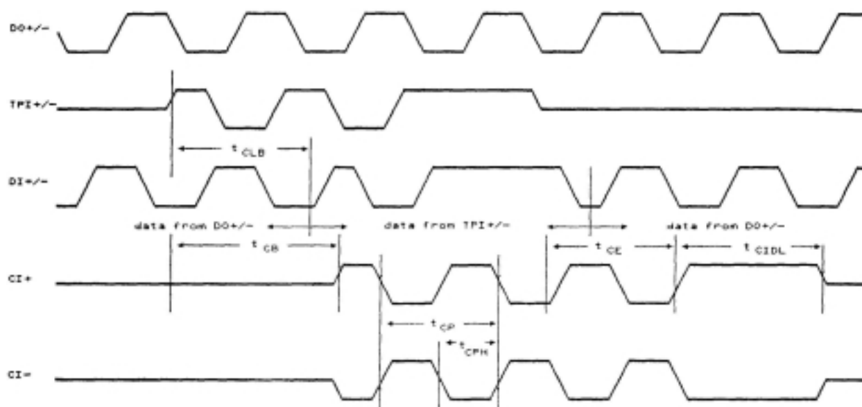
Figure 8. Collision timing
