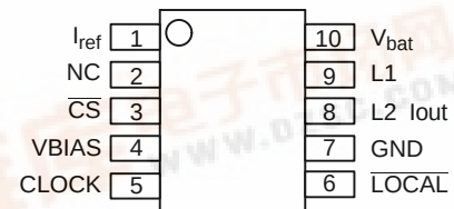
NCP5008
