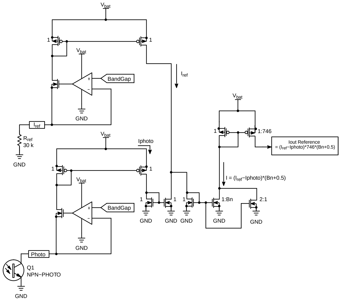
Figure 20. Functional Diagram
