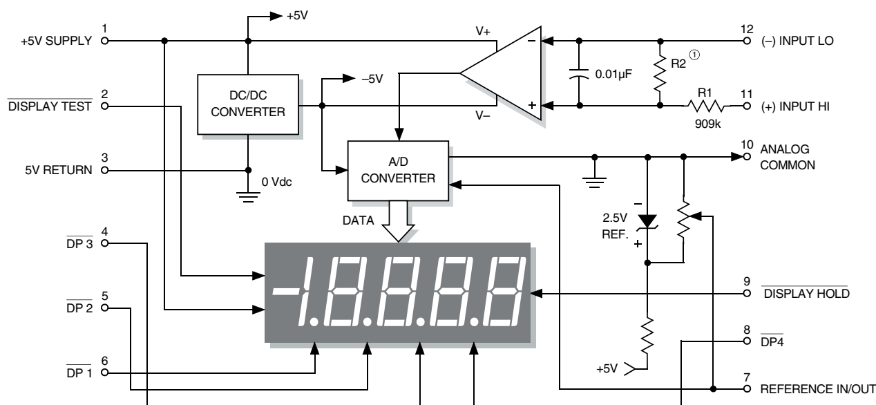
Figure 1. DMS-40PC Series Simplified Schematic
