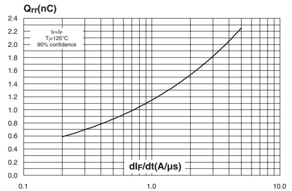
Figure 8: Reverse recovery charges versus diF/dt (damper diode)
