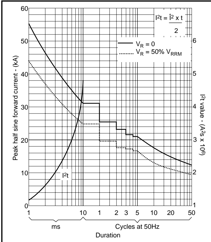
Fig.4 Surge (non-repetitive) forward current vs time at T_{case} 150°C)
