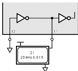
FIGURE 2. DP83910A Connection for Oscillator Module
