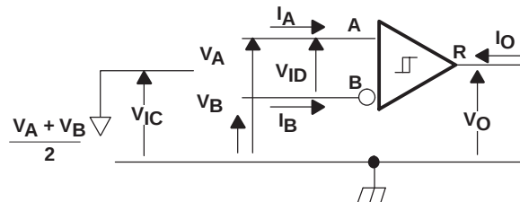
Figure 9. Receiver DC Parameter Definitions
