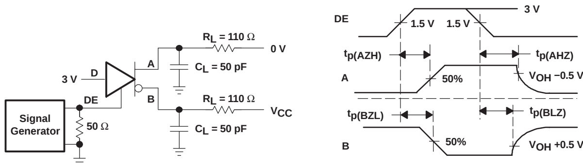
b) D at Logic High
