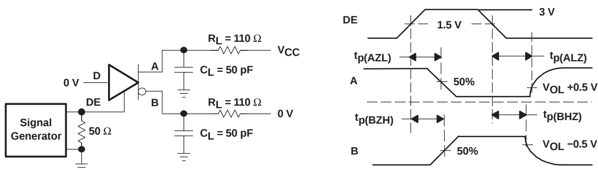
a) D at Logic Low
