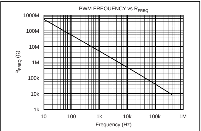
FIGURE 4. Using a Resistor to Program Oscillator Frequency. R FREQ (kΩ) = 6808417/F (1.0288)
