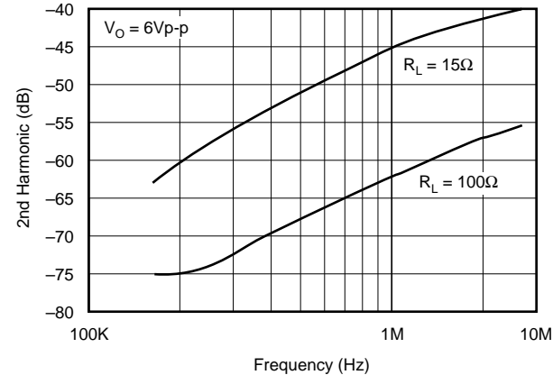
LARGE SIGNAL 2ND HARMONIC DISTORTION
