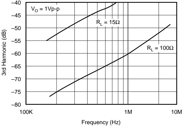
SMALL SIGNAL 3RD HARMONIC DISTORTION
