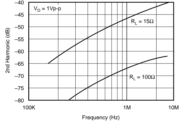
SMALL SIGNAL 2ND HARMONIC DISTORTION
