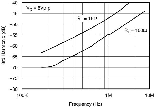
LARGE SIGNAL 3RD HARMONIC DISTORTION
