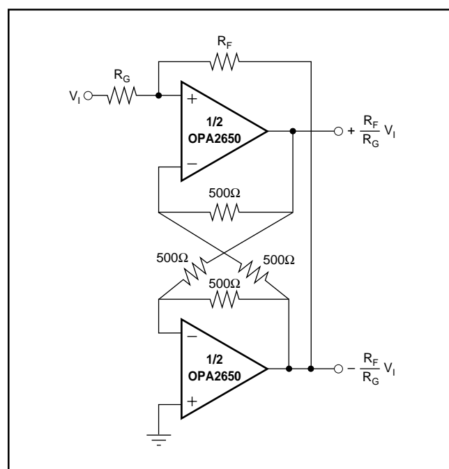
FIGURE 6. Single Ended to Differential Conversion.
