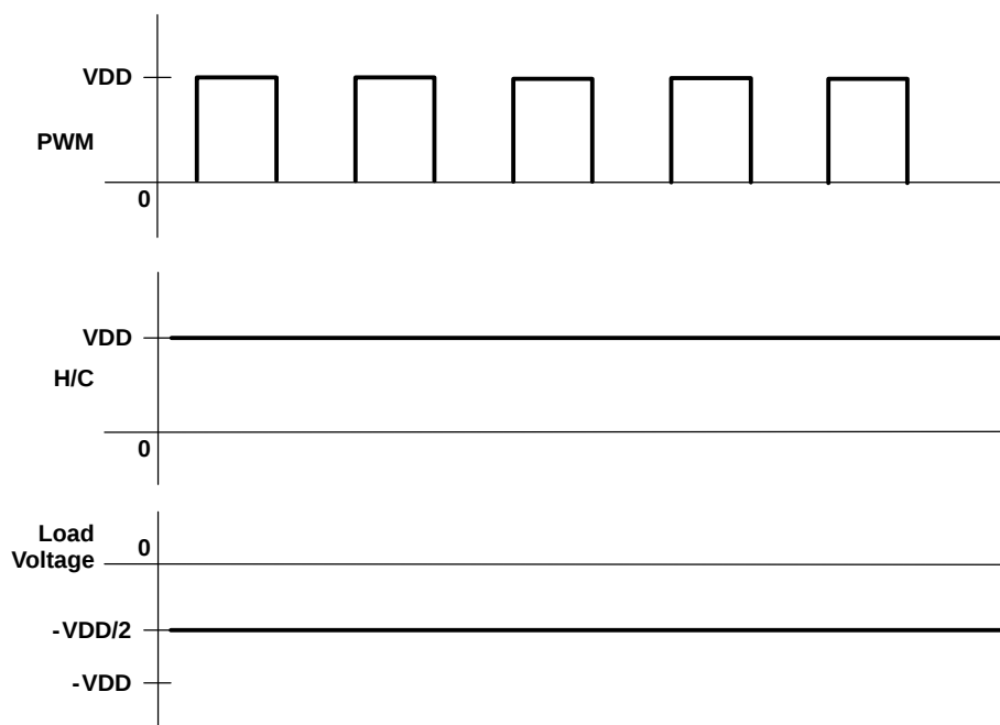
Figure 19. Heating Mode
