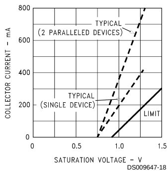
Collector Current vs Saturation Voltage
