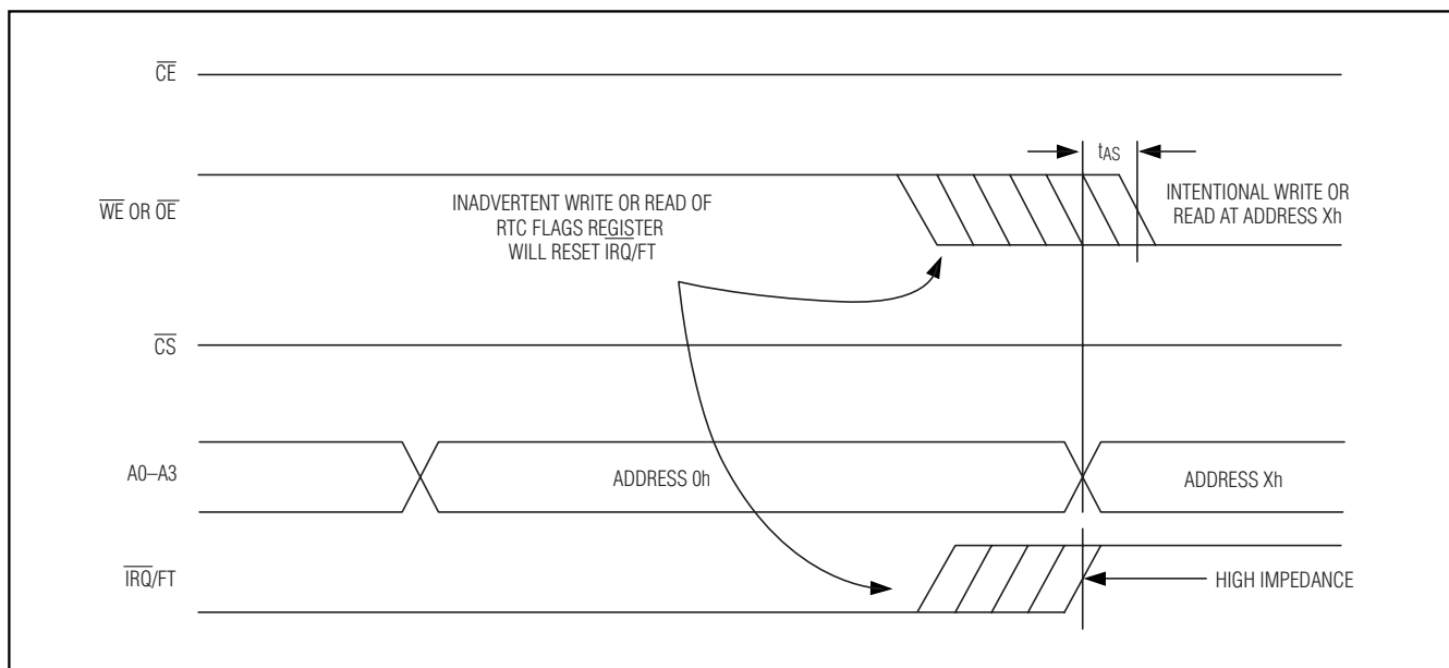
Figure 2. Prevent Accidental Clearing of IRQ Waveforms
