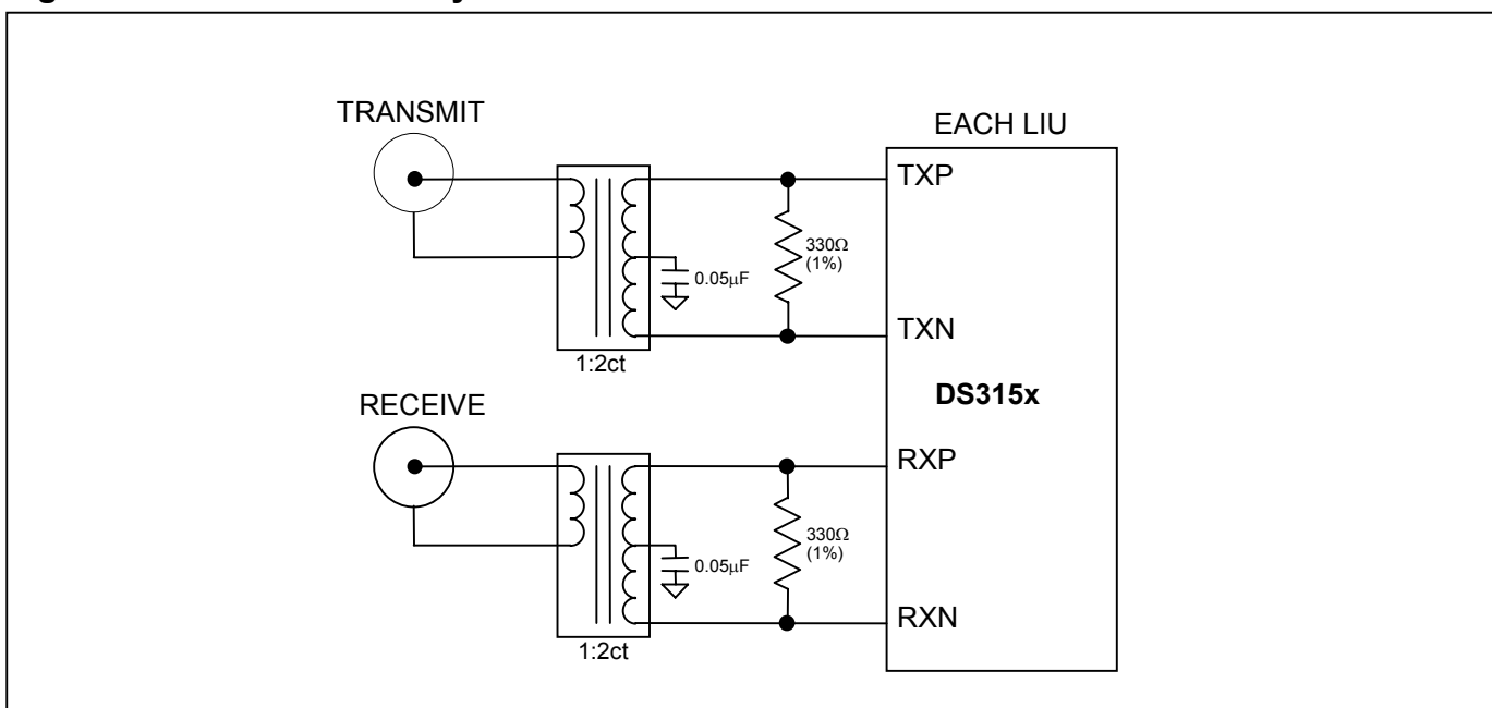
Figure 3. Line-Side Circuitry
