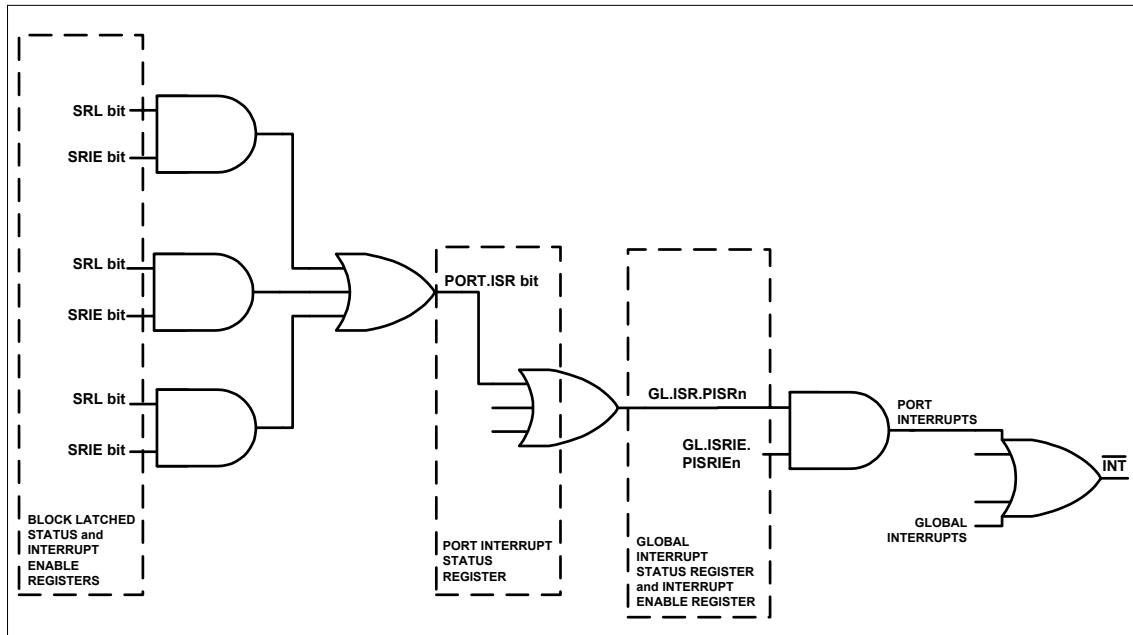
Figure 10-1. Interrupt Structure
