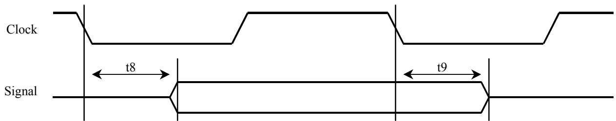
Figure 18-6. To/From Hi Z Delay Definitions (Falling Clock Edge)
