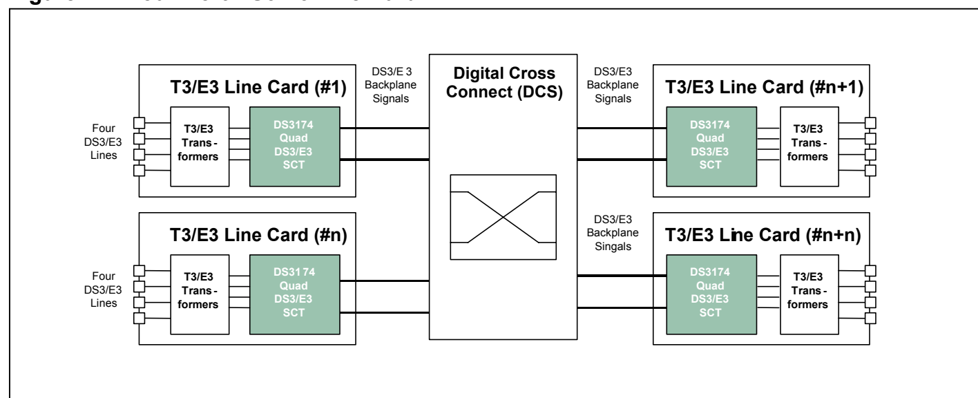
Figure 2-1. Four-Port DS3/E3 Line Card
