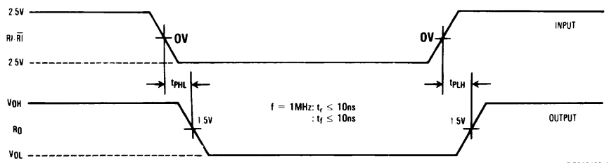
FIGURE 3. Receiver Input-to-Output Propagation Delay Timing
