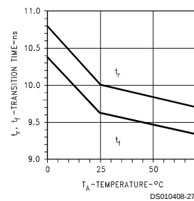
Driver Transition Time vs Temperature
