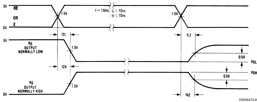
FIGURE 3. Receiver Enable/Disable Propagation Delay Timing
