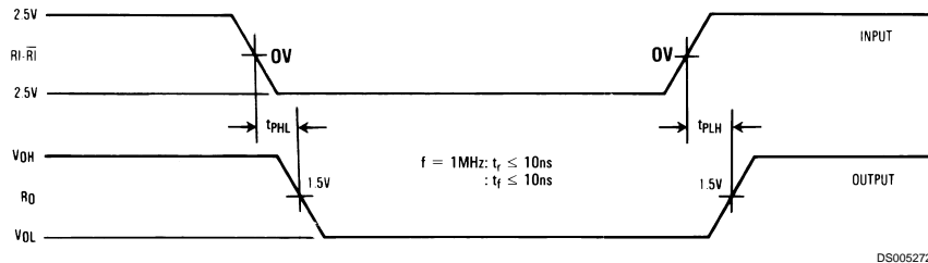
FIGURE 2. Receiver Input-to-Output Propagation Delay Timing
