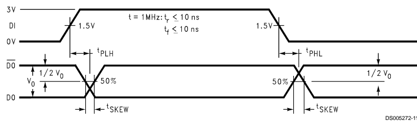
FIGURE 5. Driver Input-to-Output Propagation Delay Timing (Single-Ended)
