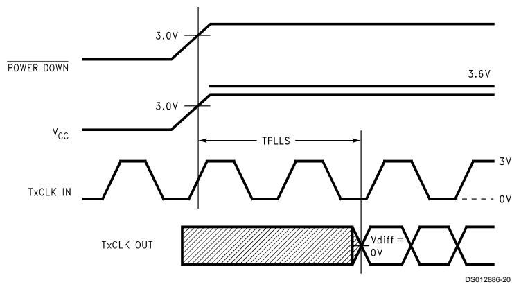
FIGURE 11. DS90C363 (Transmitter) Phase Lock Loop Set Time
