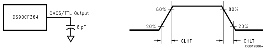
FIGURE 4. DS90CF364 (Receiver) CMOS/TTL Output Load and Transition Times
