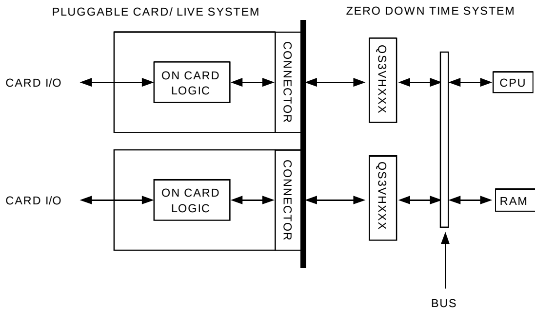
Hot-Swapping
