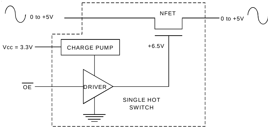
Rail-to-Rail Switching
