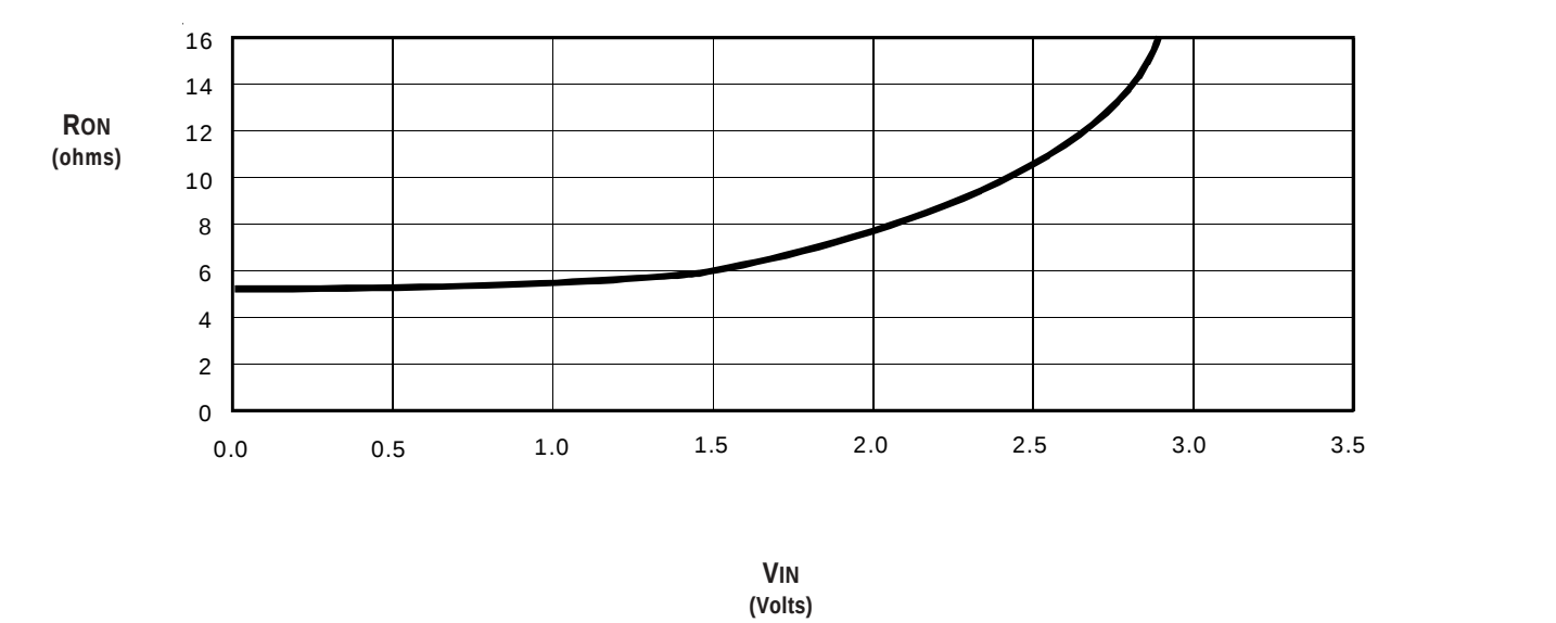
TYPICAL ON RESISTANCE vs VIN AT VCC = 5V
