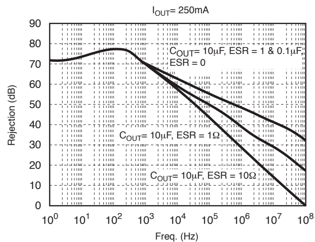
Ripple Rejection
