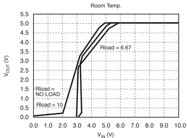
V_{OUT} vs. V_{IN} over R_{LOAD}
