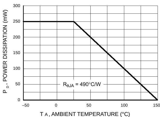
Figure 1. Derating Curve
