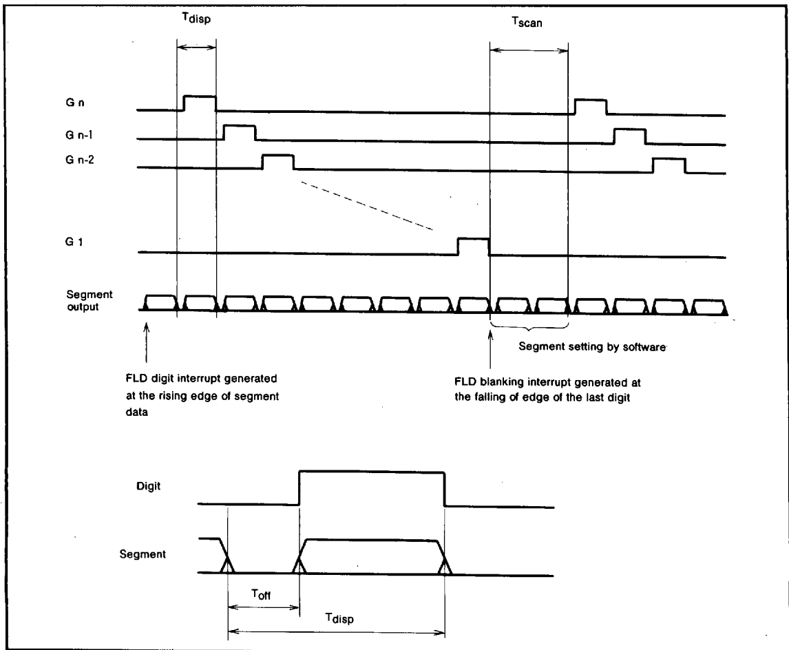
Fig. 33 FLD timing
