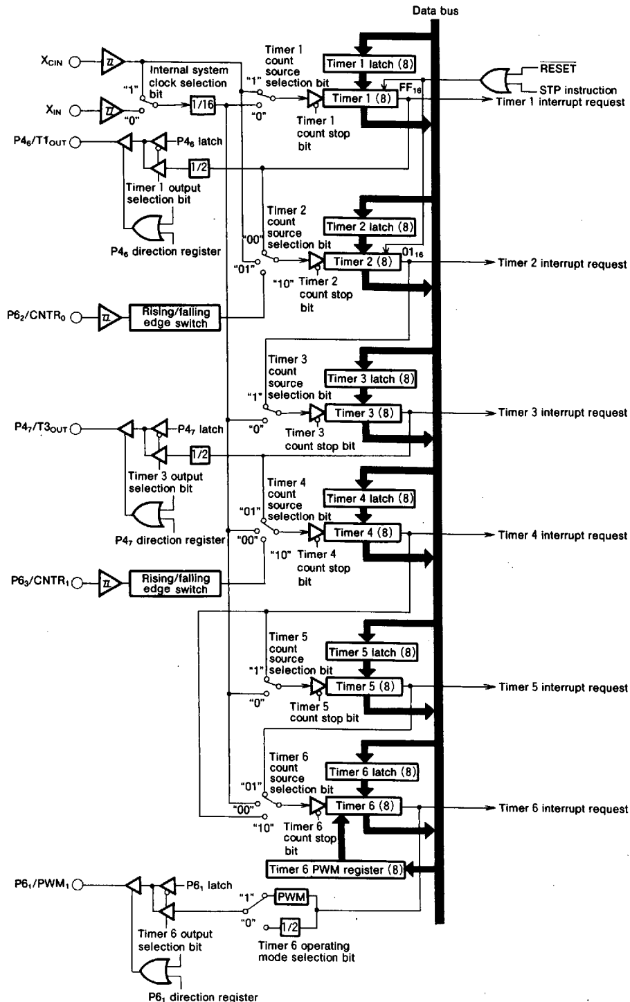
Fig. 8 Timer block diagram
