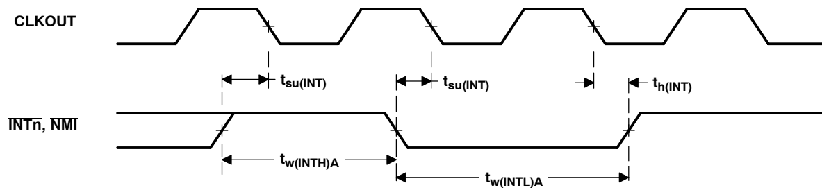
Figure 5-15. Interrupt Timing
