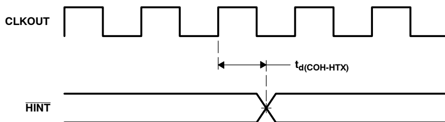
Figure 5-30. \overline{\text{HINT}} Timing
