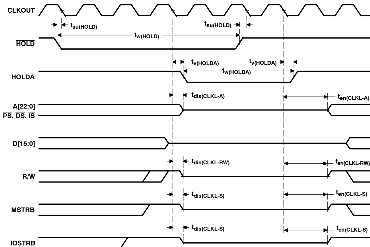
Figure 5–13. \overline{\text{HOLD}} and \overline{\text{HOLDA}} Timings
