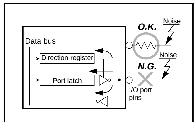
Fig. 3.4.7 Setup for I/O ports
