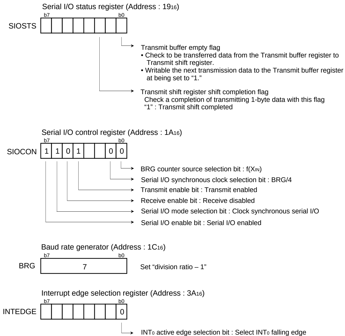
Fig. 2.3.15 Setting of related registers at a transmitting side [Communication using a clock synchronous serial I/O]
