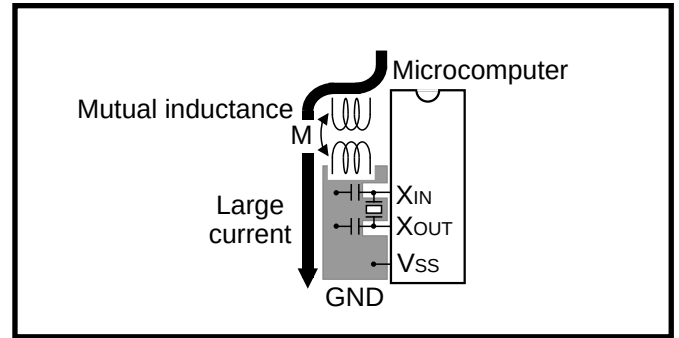
Fig.3.4.5 Wiring for a large current signal line
