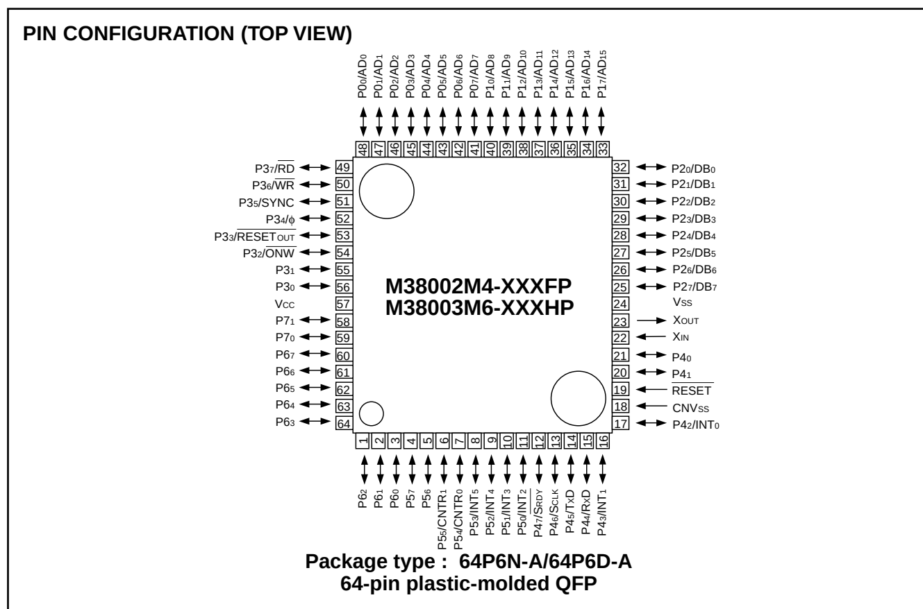
Fig. 1 Pin configuration of M38002M4-XXXXFP/M38003M6-XXXXHP
