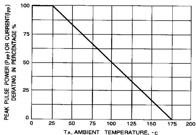
Fig. 2-PULSE DERATING CURVE
