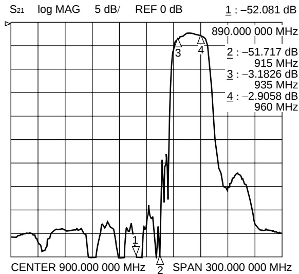
Filter 1 (Passband: 935 to 960 MHz)
