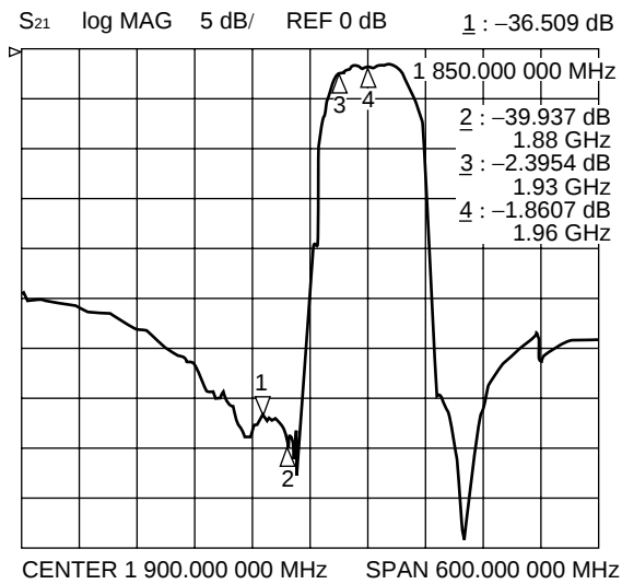
Filter 1 (Passband: 1930 to 1960 MHz)
