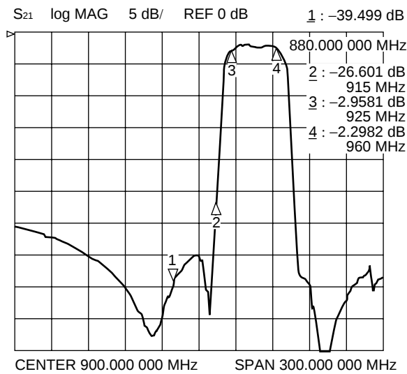
Filter 1 (Passband: 925 to 960 MHz)
