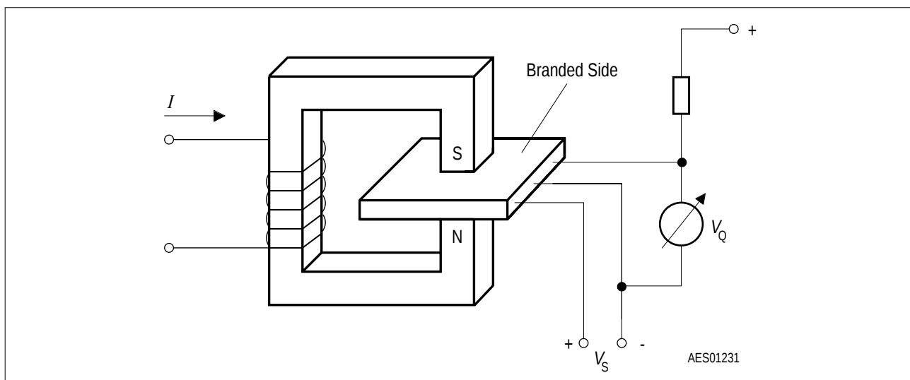
Figure 3 Sensor/Magnetic-Field Configuration
