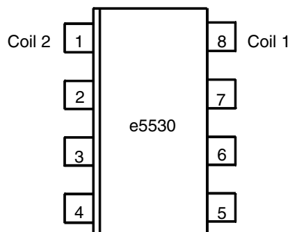
Figure 4. Pinning SO8
