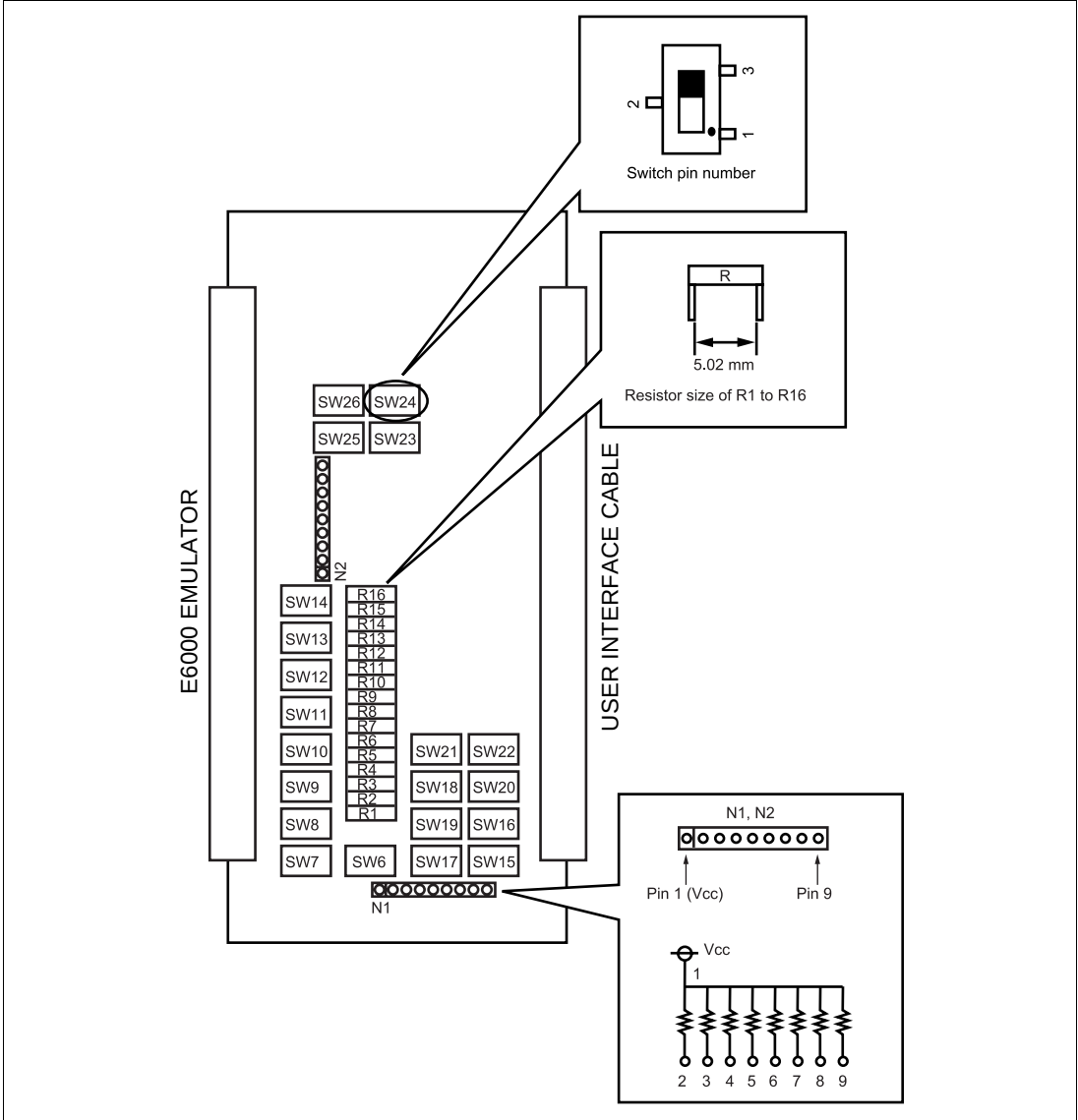
Figure 3.3 Location of Switches and Resistor
