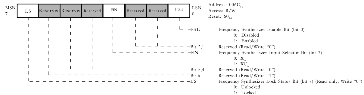
Fig. 1.93. Frequency Synthesizer Control Register (FSC)
