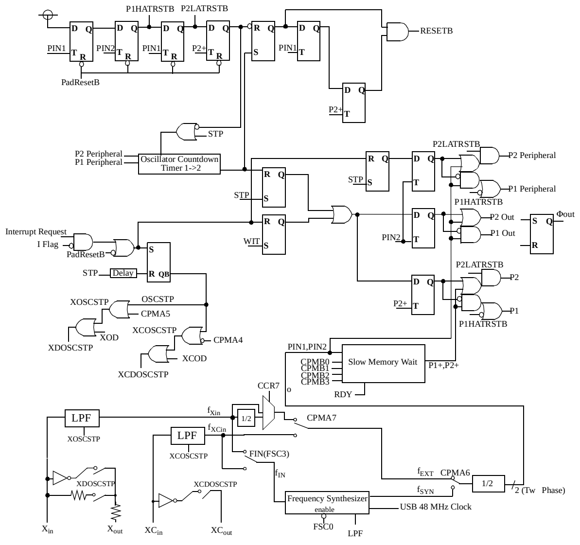
Fig. 1.92. Clock Block Diagram
