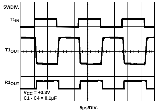
FIGURE 12. LOOPBACK TEST AT 120kbps
