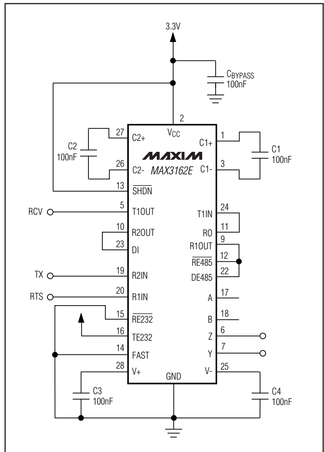
Figure 18. Protocol Translator
