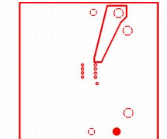
Third Layer (VCC and Ground Plane)
