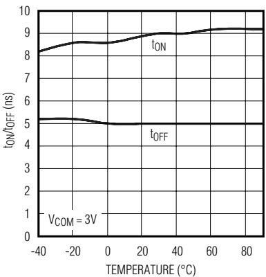
TURN-ON/TURN-OFF TIMES vs. TEMPERATURE
