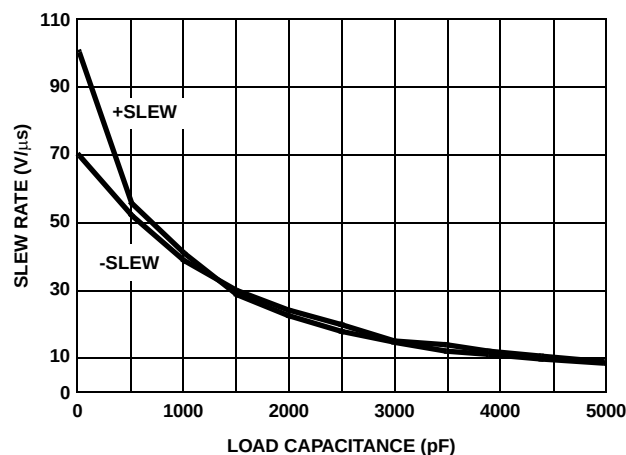
FIGURE 24. ISL4245E SLEW RATE vs LOAD CAPACITANCE
