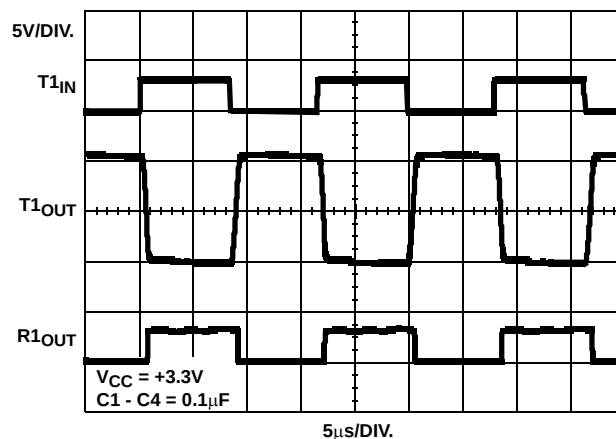
FIGURE 13. ISL4238E/44E LOOPBACK TEST AT 120kbps
