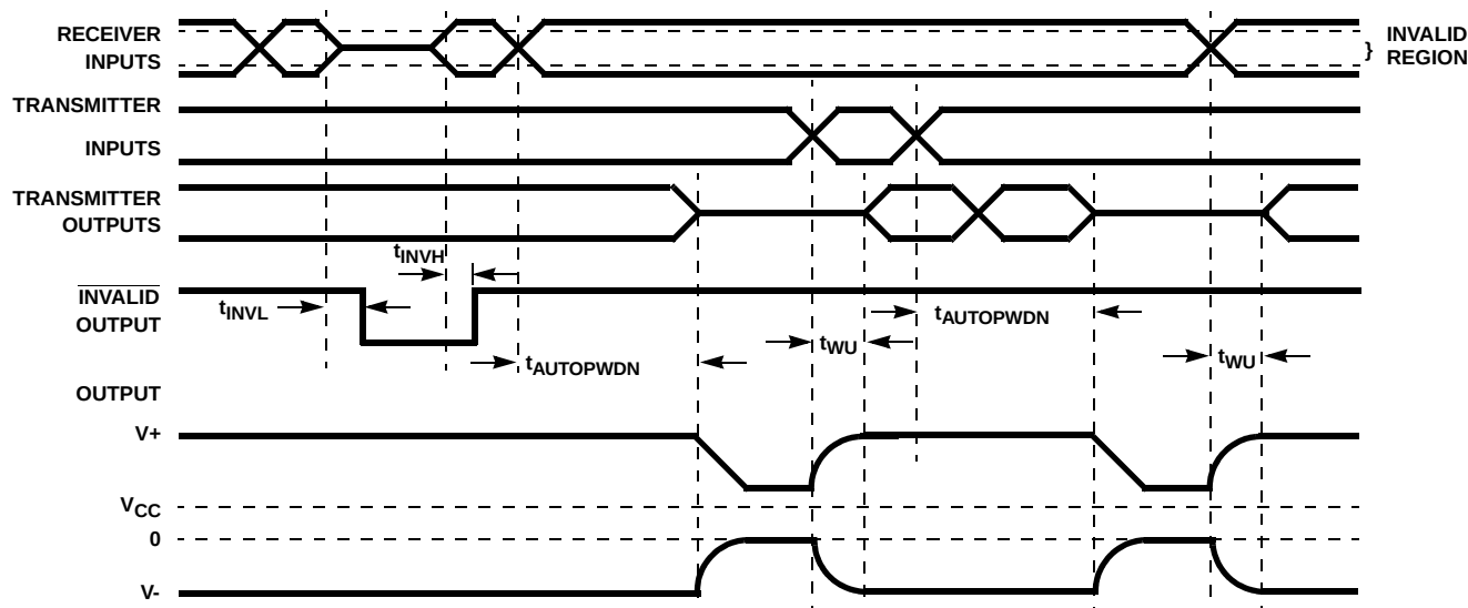
FIGURE 9. ENHANCED AUTOMATIC POWERDOWN AND INVALID TIMING DIAGRAMS
