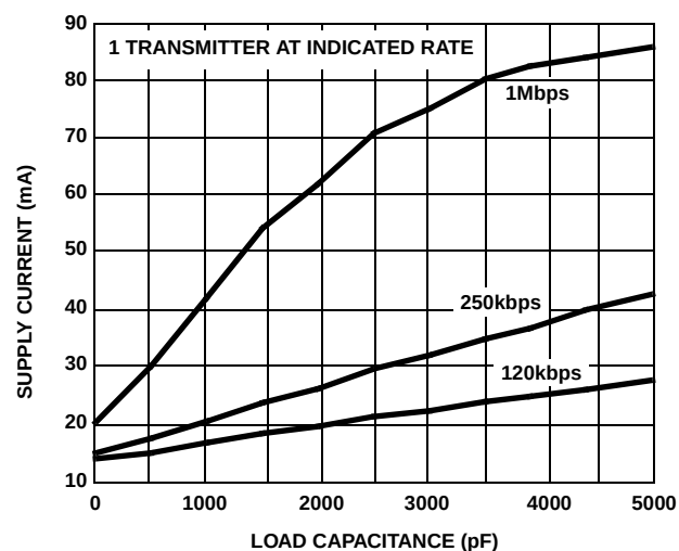
FIGURE 22. ISL4245E SUPPLY CURRENT vs LOAD CAPACITANCE WHEN TRANSMITTING DATA
