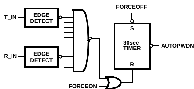
FIGURE 7. ENHANCED AUTOMATIC POWERDOWN LOGIC on the state of the ISL4238E/4XE (see the next sections for methods of utilizing \overline{\text{INVALID}} to power down the device).
