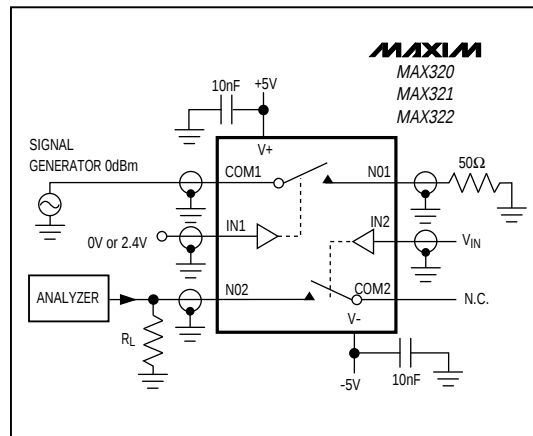
Figure 6. Crosstalk
