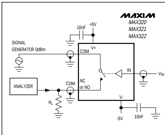
Figure 5. Off Isolation
