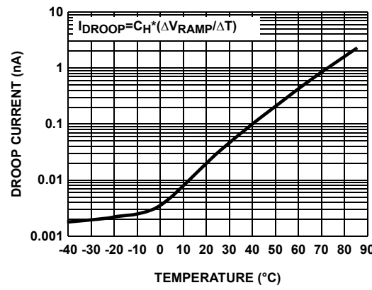
FIGURE 19. DROOP CURRENT vs TEMPERATURE
