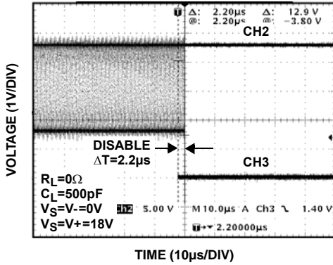
FIGURE 7. DISABLE RESPONSE
