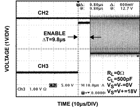
FIGURE 8. ENABLE RESPONSE
