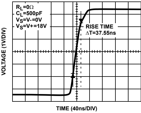
FIGURE 1. RISE TIME OUTPUT 6V p.p
