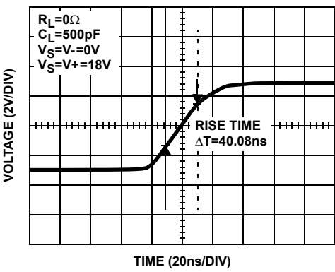
FIGURE 5. RISE TIME OUTPUT 5V p.p
