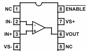
EL8178 (8 LD SO) TOP VIEW
