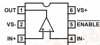
EL8178 (6 LD SOT-23) TOP VIEW
