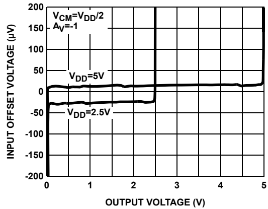
FIGURE 4. INPUT OFFSET VOLTAGE vs OUTPUT VOLTAGE
