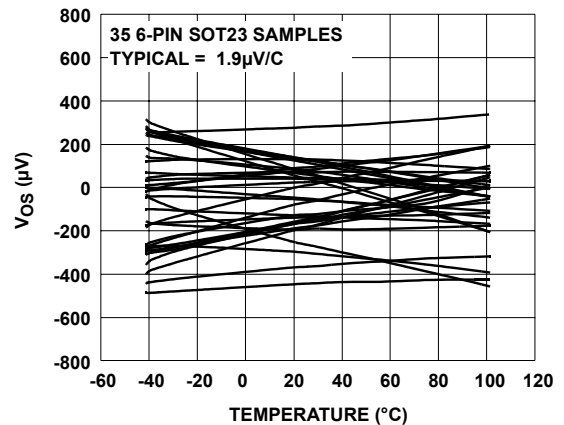
FIGURE 12. SOT V_{OS} vs TEMPERATURE ( V_S = 5V )
