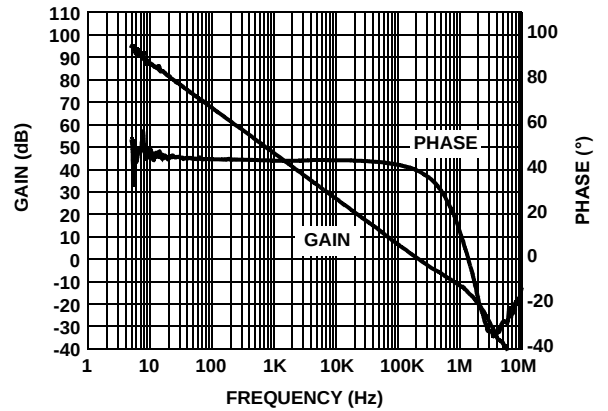
FIGURE 8. OPEN LOOP GAIN AND PHASE vs FREQUENCY @ 100kΩ
