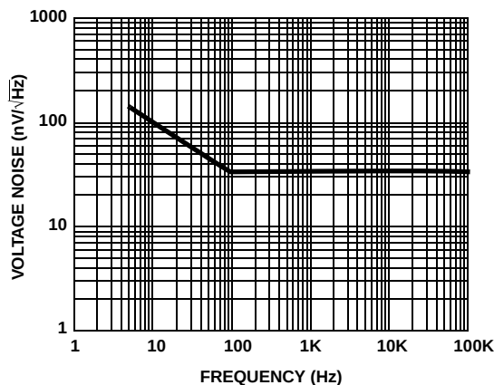
FIGURE 11. VOLTAGE NOISE
