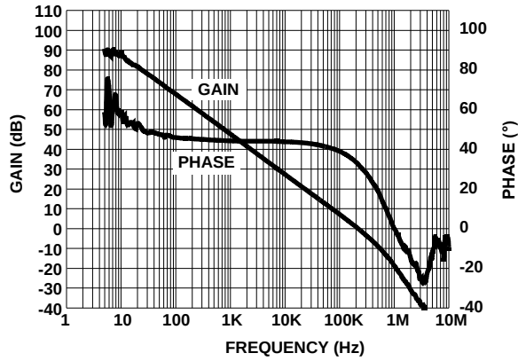
FIGURE 7. OPEN LOOP GAIN vs FREQUENCY @ 1kΩ
