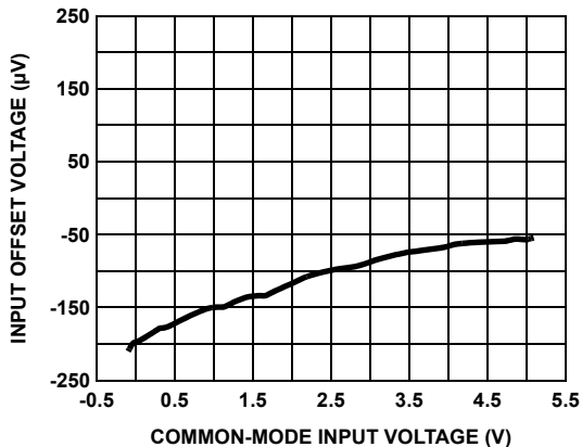
FIGURE 5. INPUT OFFSET VOLTAGE vs COMMON-MODE INPUT VOLTAGE
