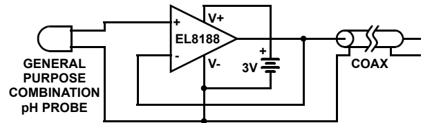
FIGURE 16. PH PROBE AMPLIFIER
