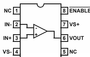
EL8188 (8-PIN SO) TOP VIEW
