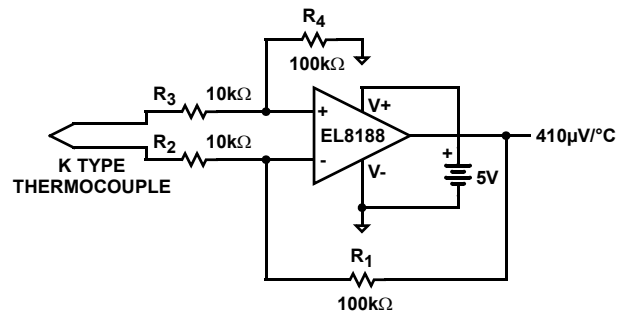
FIGURE 17. THERMOCOUPLE AMPLIFIER
