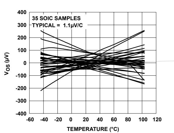
FIGURE 13. SOIC V_{OS} vs TEMPERATURE ( V_S = 5V )
