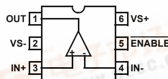
EL8188 (6-PIN SOT-23) TOP VIEW
