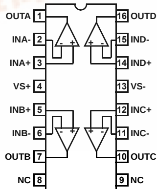
EL8401 (16-PIN QSOP) TOP VIEW
