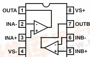
EL8201 (8-PIN SO) TOP VIEW
