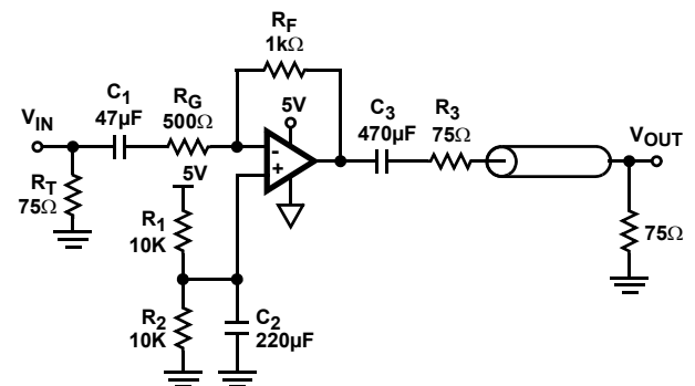
FIGURE 34. 5V SINGLE SUPPLY INVERTING VIDEO LINE DRIVER
