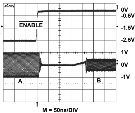
FIGURE 32. ENABLE SIGNAL
