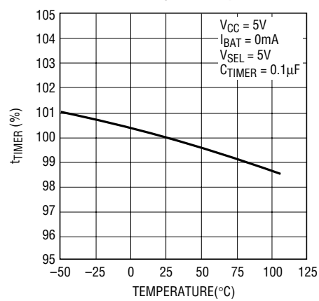
Timer Accuracy vs Temperature
