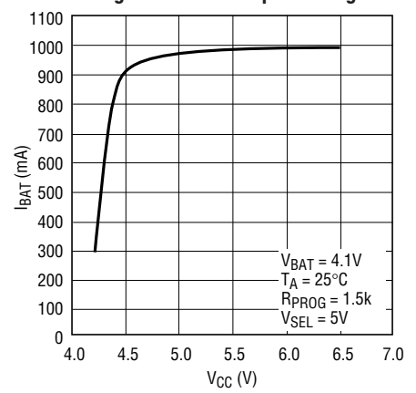
Charge Current vs Input Voltage
