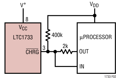
Figure 2. Microprocessor Interface
