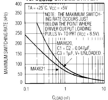
MAXIMUM SWITCHING RATE vs. LOAD SINGLE DRIVER
